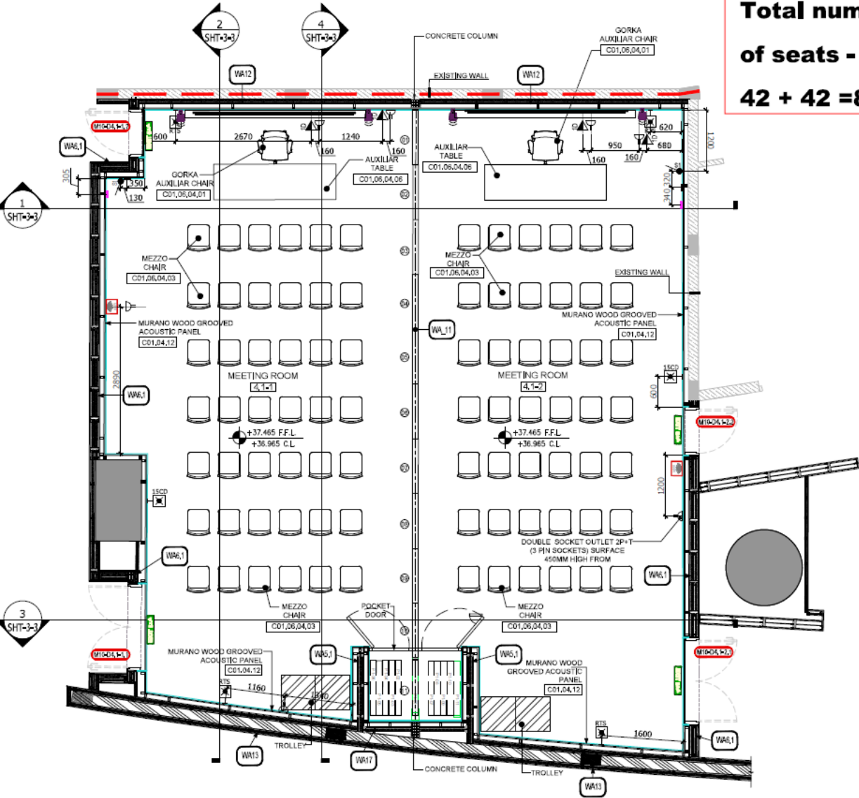
1 SETTING OUT & FURNITURE LAYOUT- MEETING ROOM, LEVEL-07 MUSEUM BUILDING SCALE-1:50
