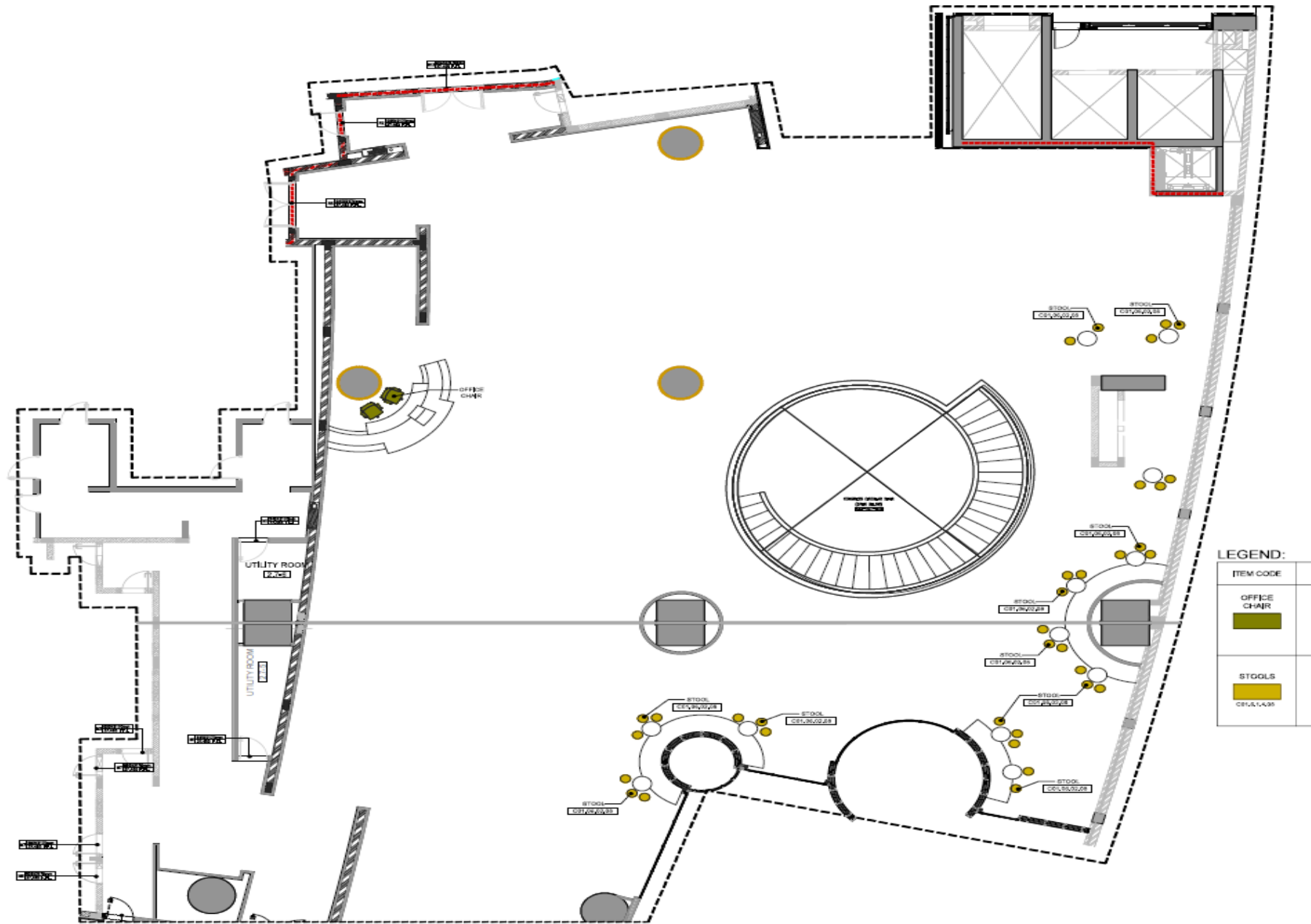
1 FURNITURE LAYOUT-HALL AREA, THIRD FLOOR SCALE: 1/16"
