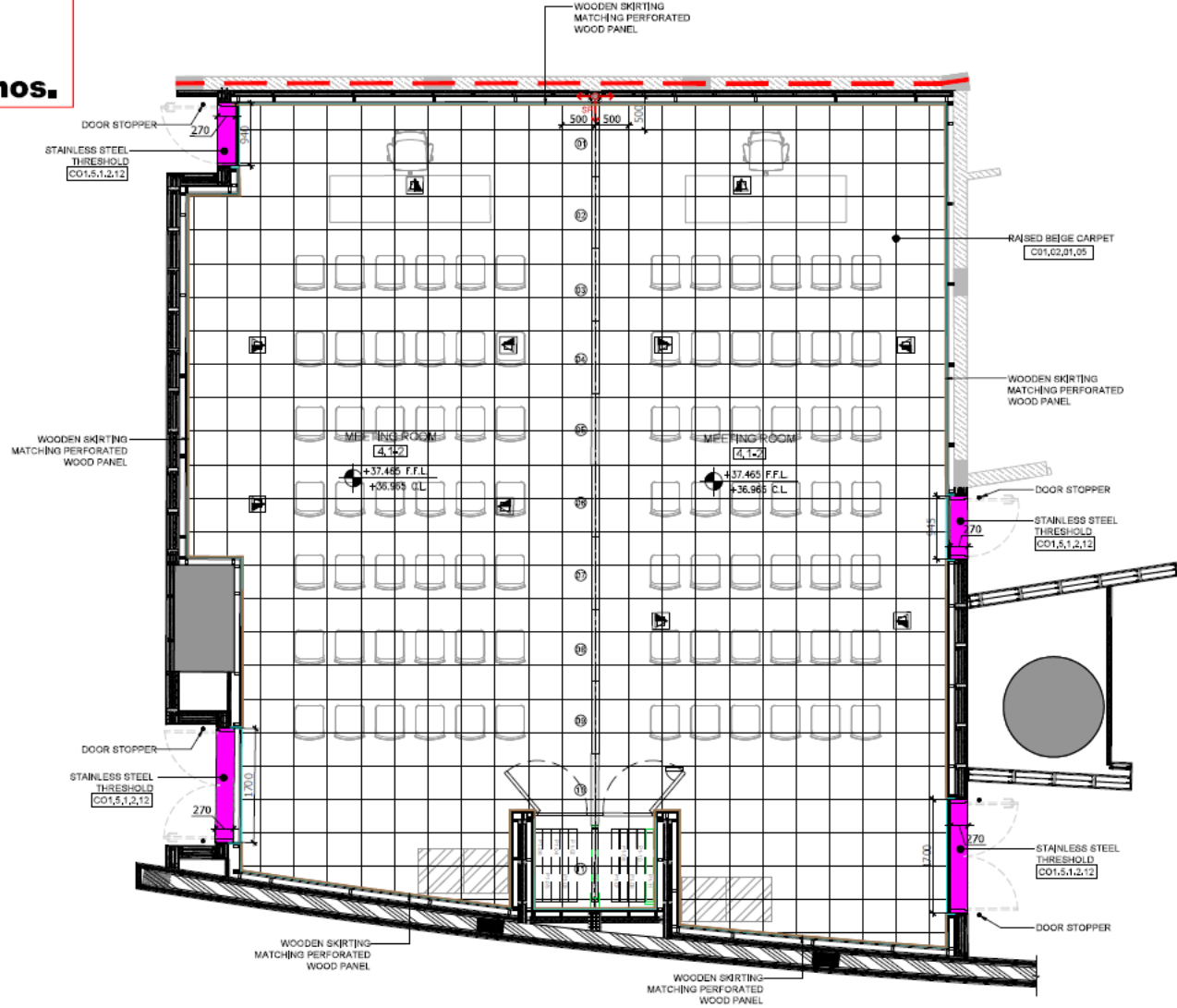
2 FLOORING LAYOUT- MEETING ROOM, LEVEL-07 MUSEUM BUILDING SCALE-1:50
